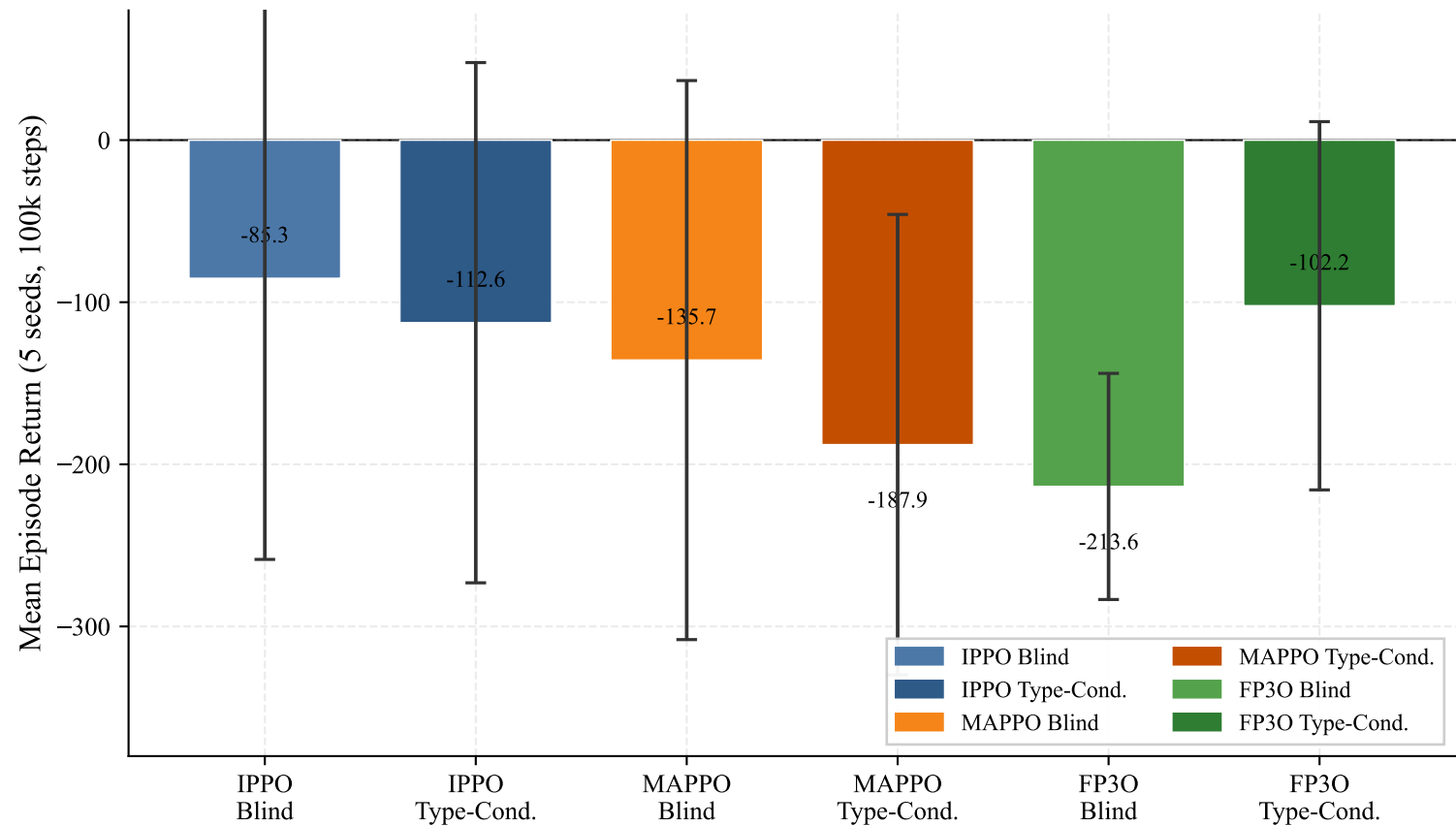
2 \times 3 Coupled-Channel Factorial: Mean Return \pm 95% CI
